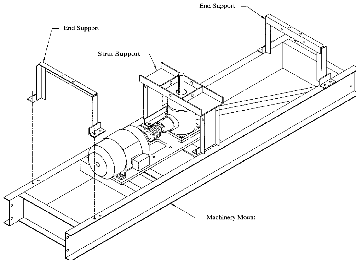
FIG. C3 - STRUT SUPPORT AND END SUPPORTS
