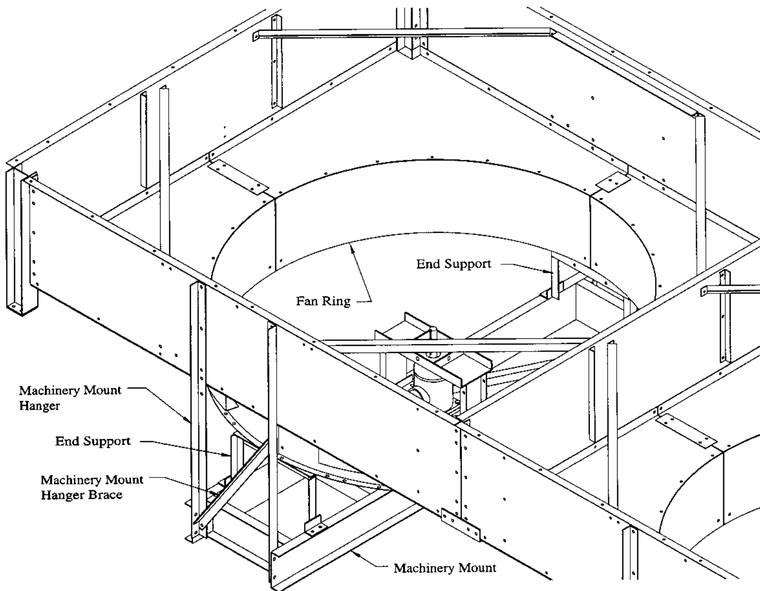
FIG. C4 - MACHINERY MOUNT
