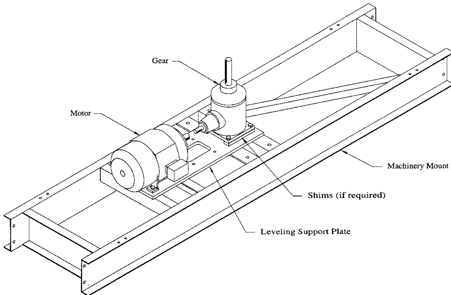
FIG. C1 - GEAR AND MOTOR
