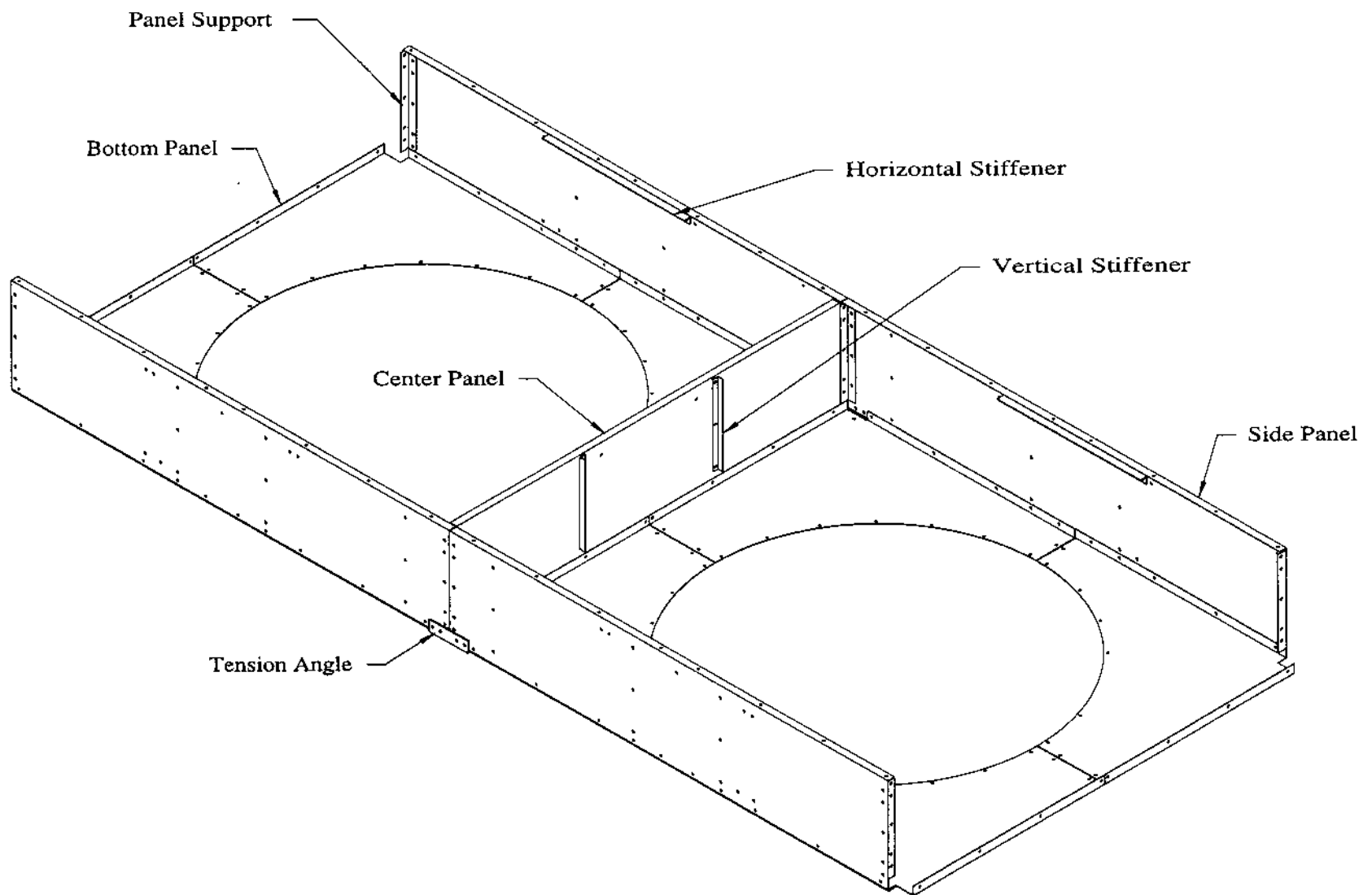
FIG. B1 - BOTTOM, CENTER, AND SIDE PANELS
