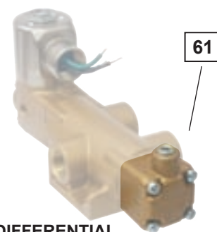
DIFFERENTIAL PILOT RETURN
